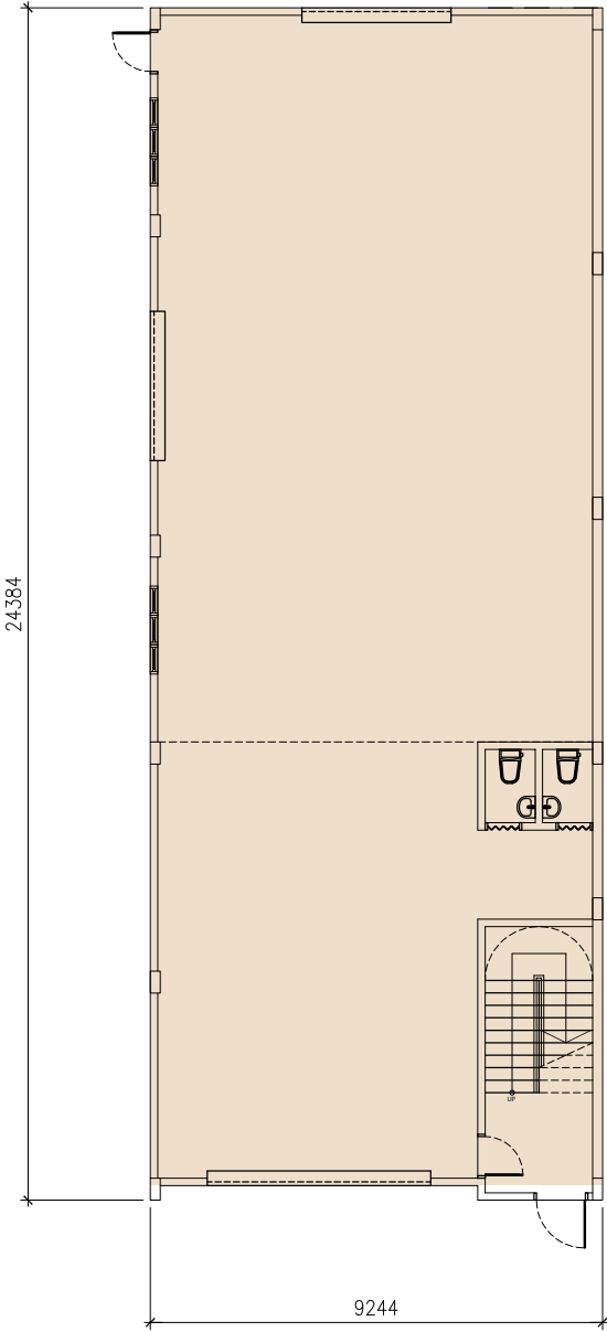
Ground Floor [30' X 80']
